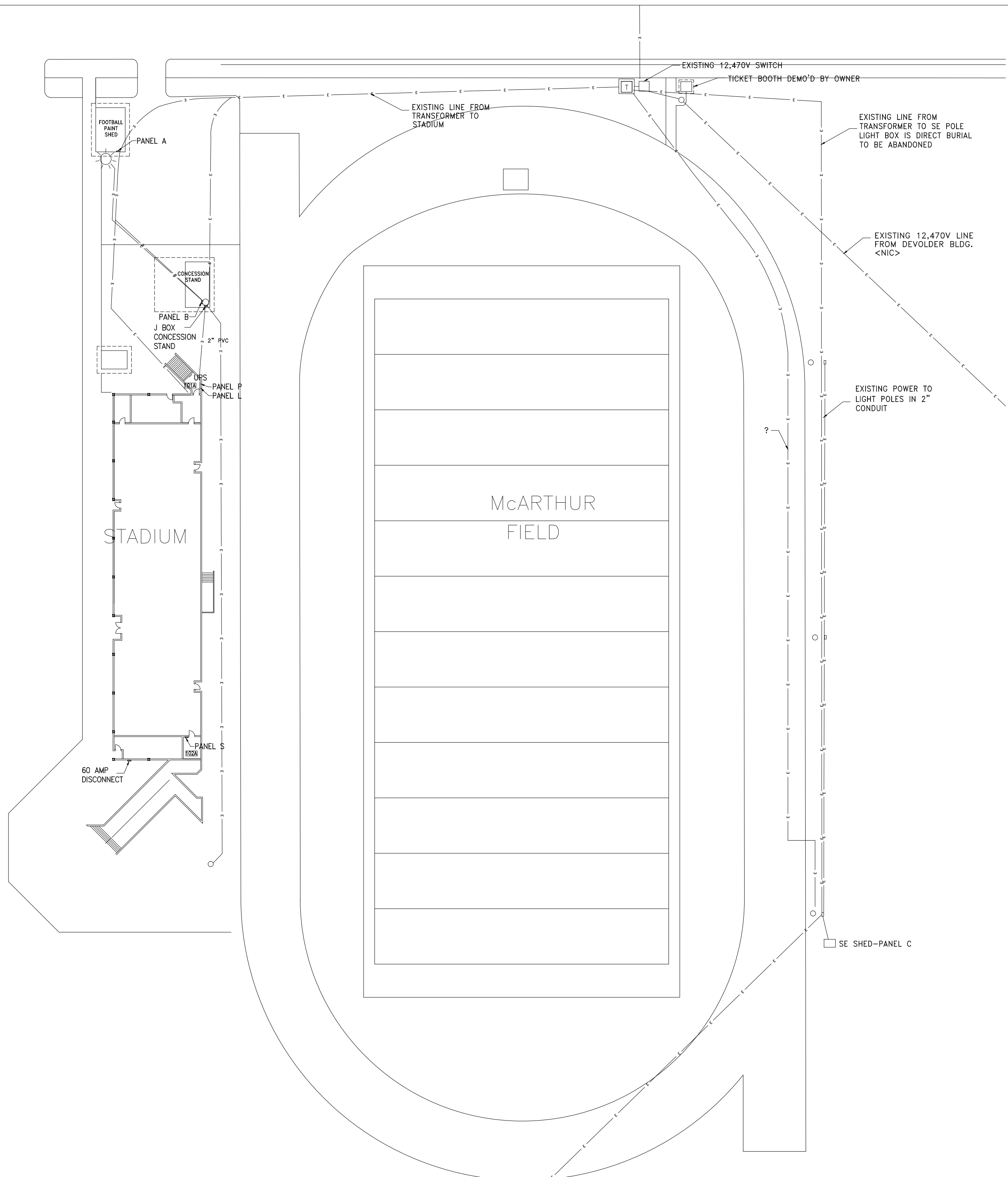
1 E1 EXISTING UTILITY PLAN/ LAYOUT SCALE: 1" = 40'
