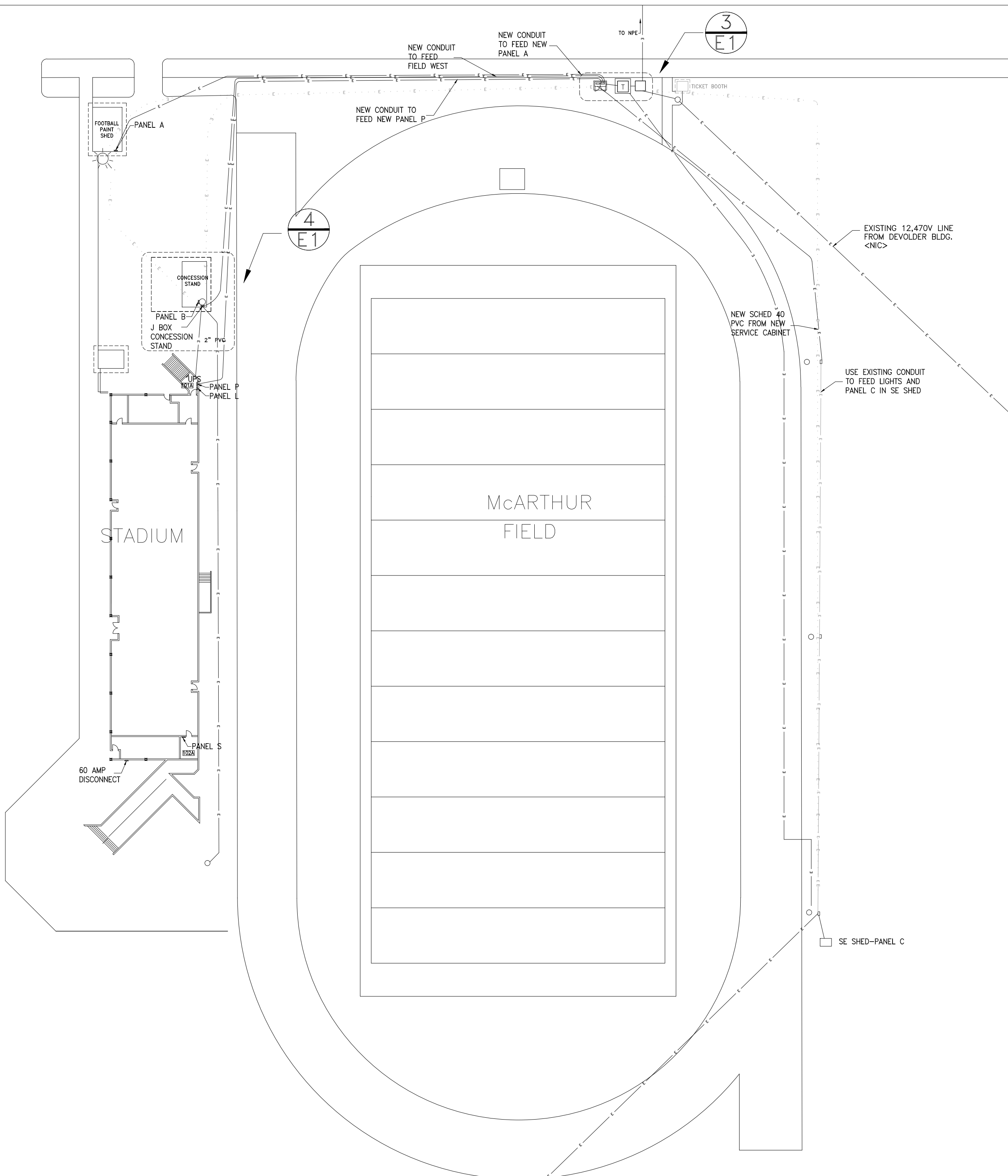
2 E1 PROPOSED UTILITY PLAN/ LAYOUT SCALE: 1" = 40"
