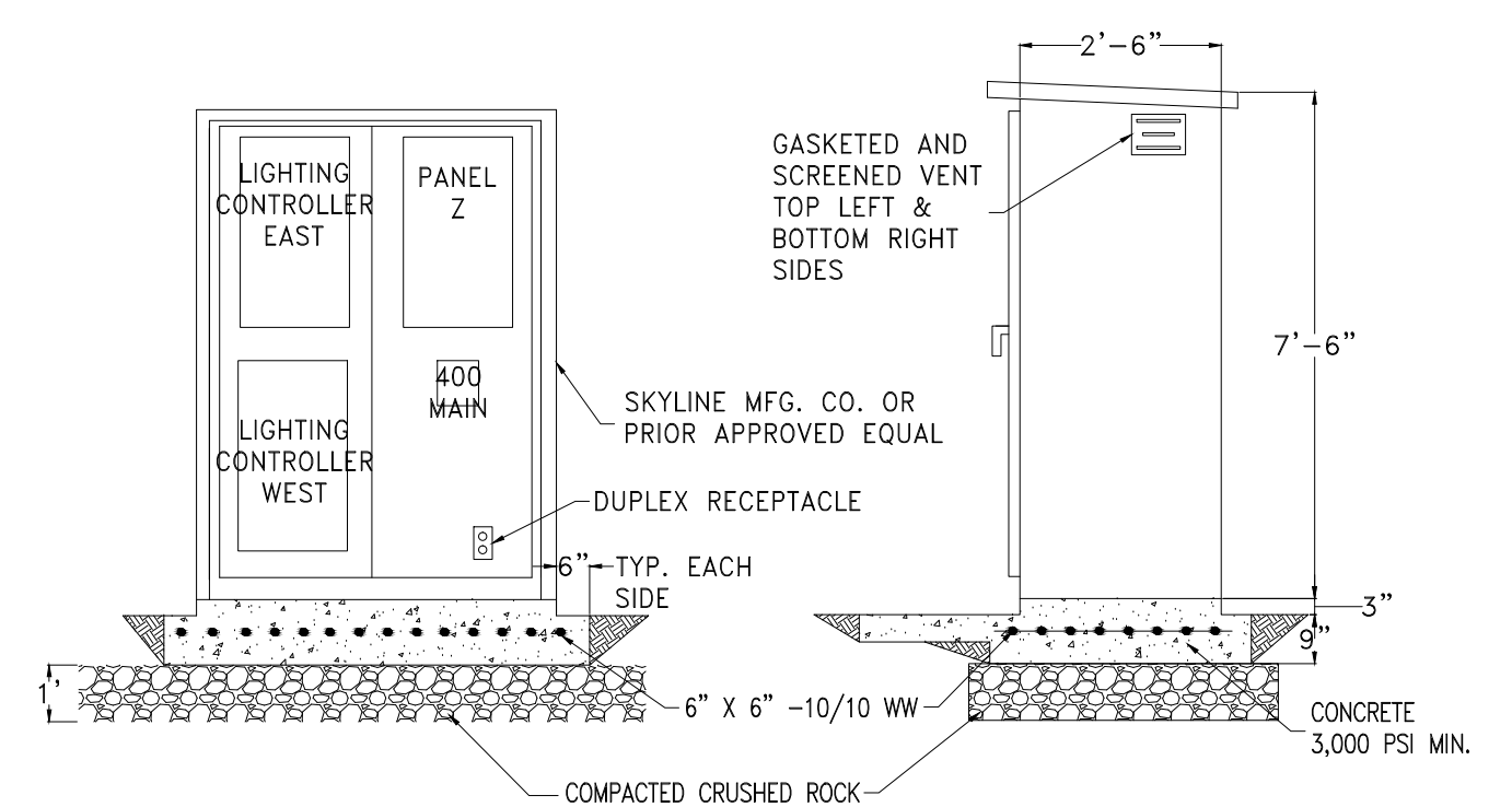
3 E1 NEW ELECTRICAL SERVICE CABINET ON NEW CONCRETE PAD DETAIL SCALE: NTS
