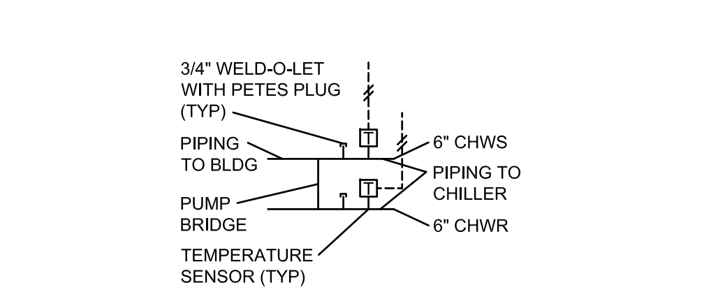
B HAMERSLY PIPING AND CONTROL SCHEMATIC NO SCALE
