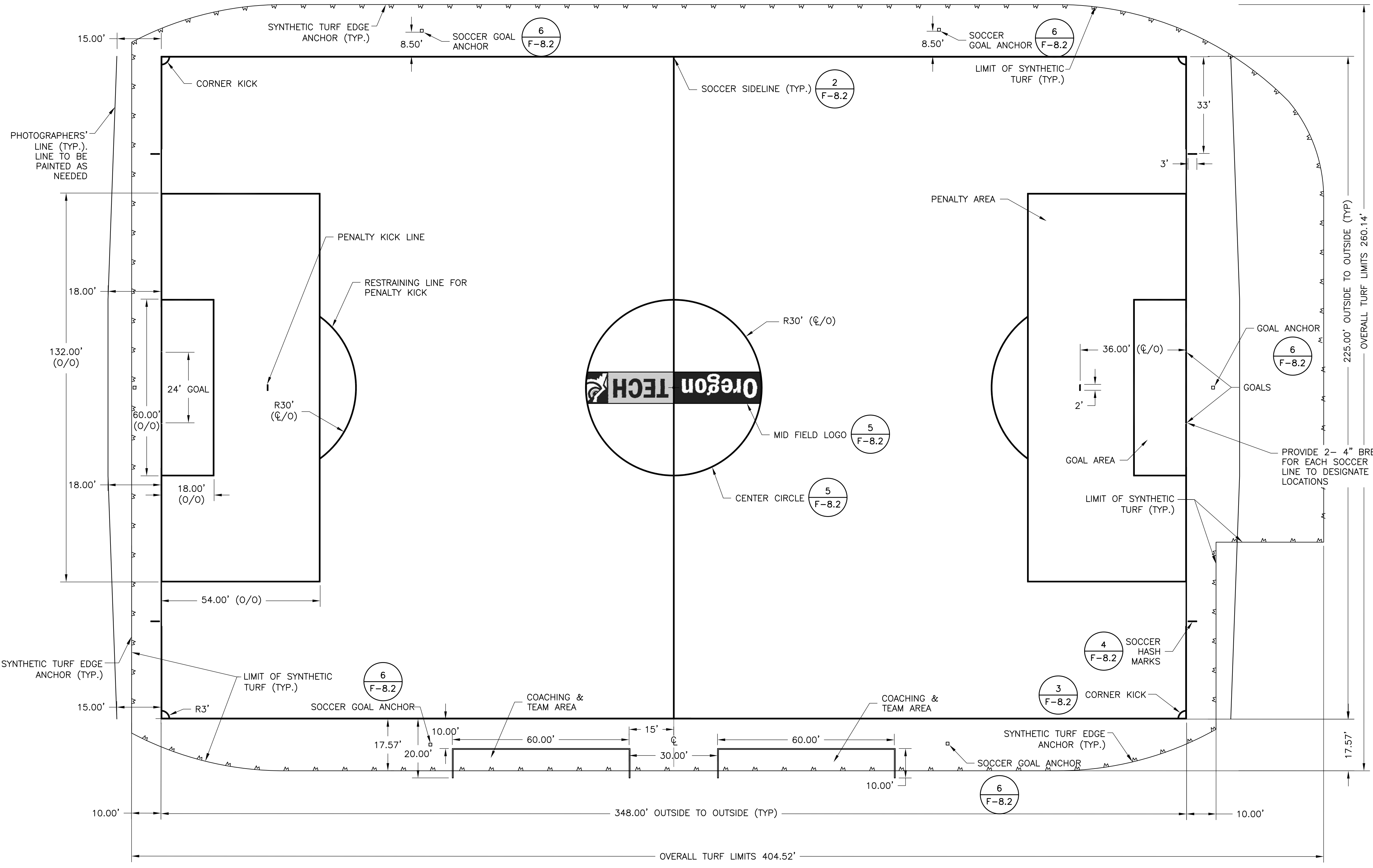
1 SOCCER LAYOUT & MARKING PLAN F-8.1 SCALE 1"=20'
