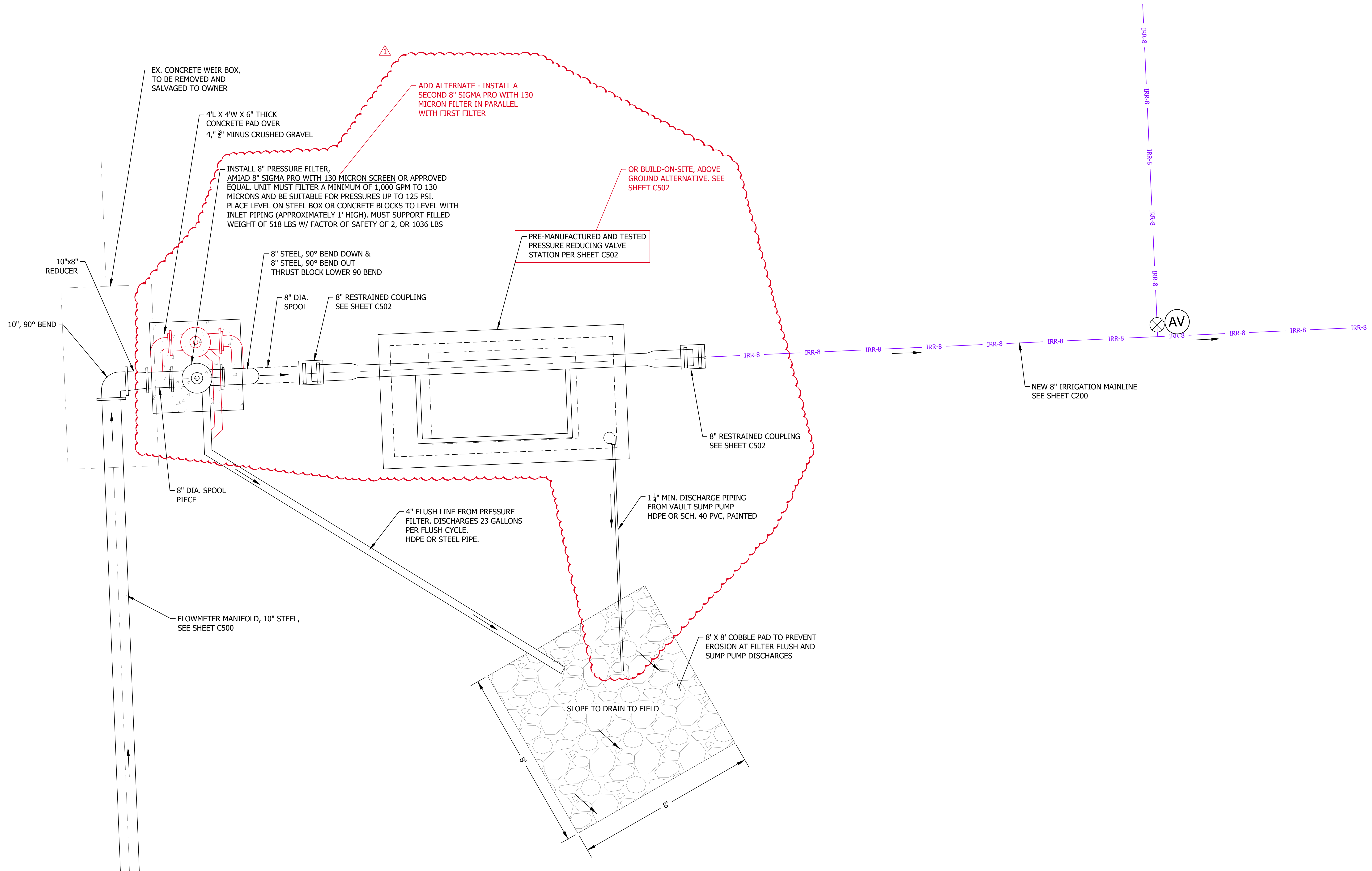
PRESSURE FILTER AND PRV STATION DETAILS
