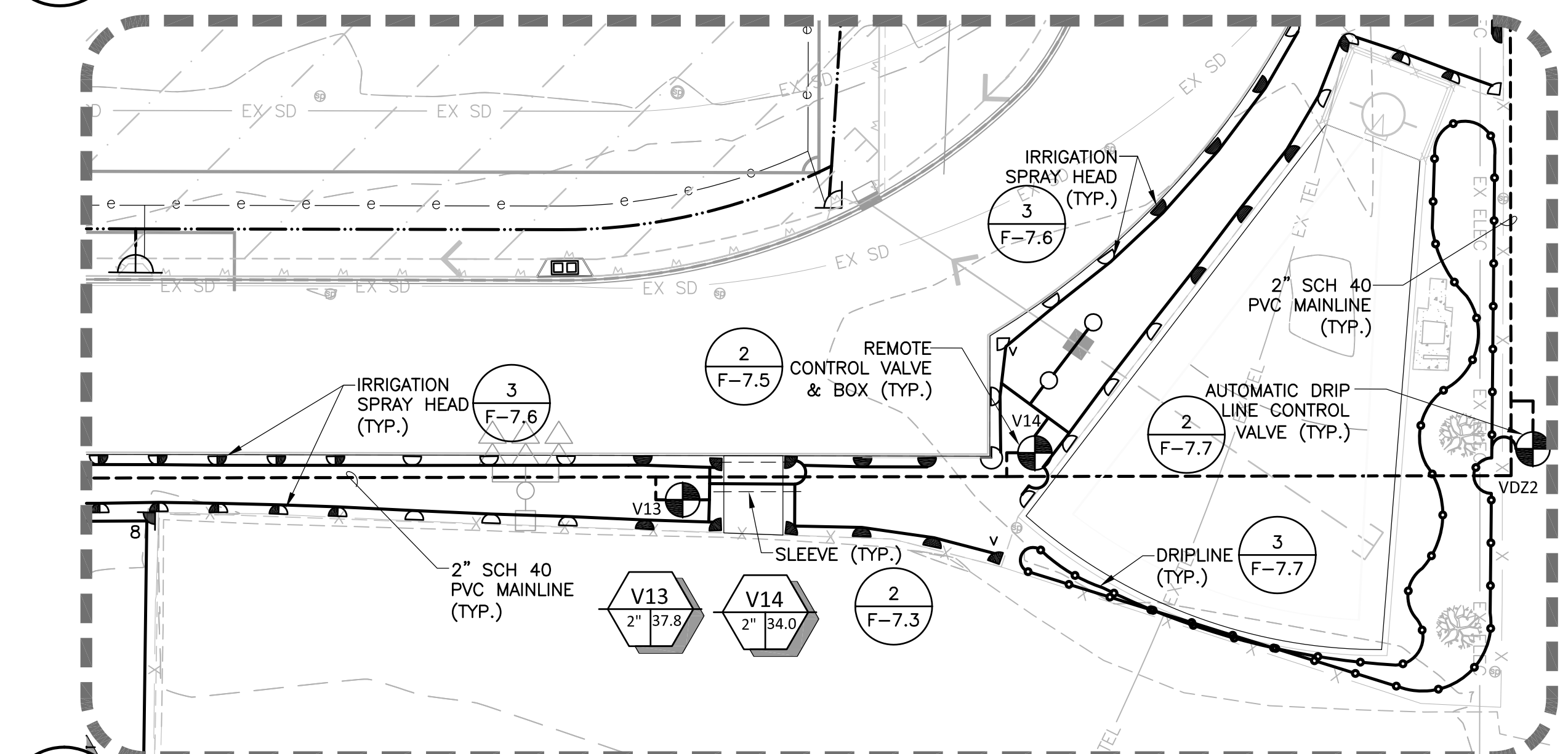
3 LANDSCAPED AREA @ FIELD EVENTS - SOUTH EAST F-5.1 AS NOTED
