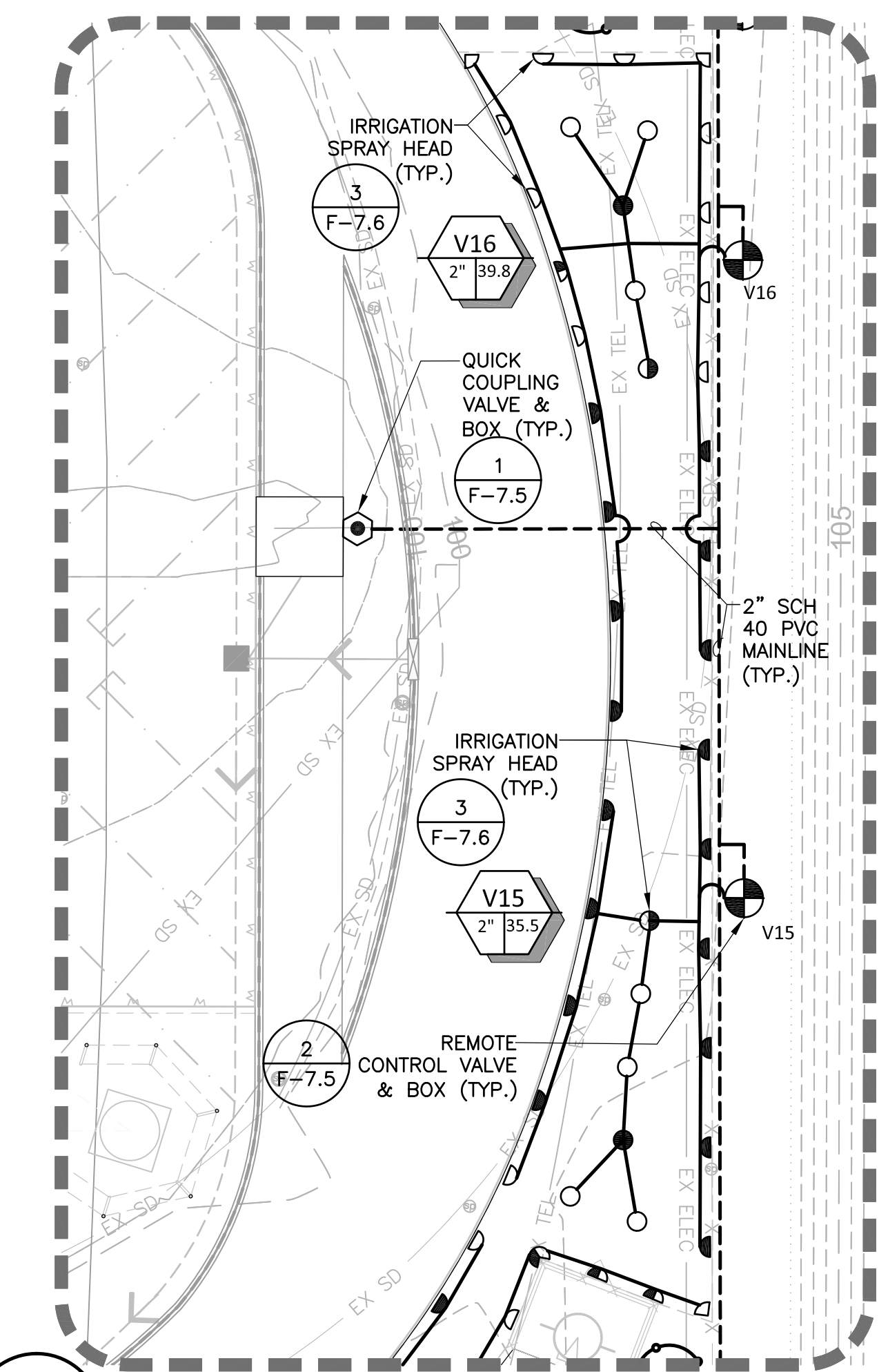
4 LANDSCAPED AREA - EAST F-5.1 AS NOTED
