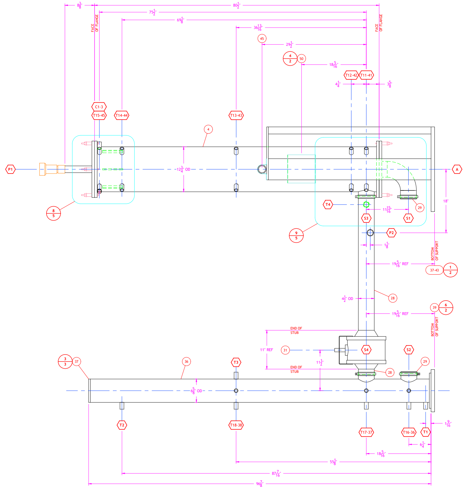
ELEVATION VIEW
