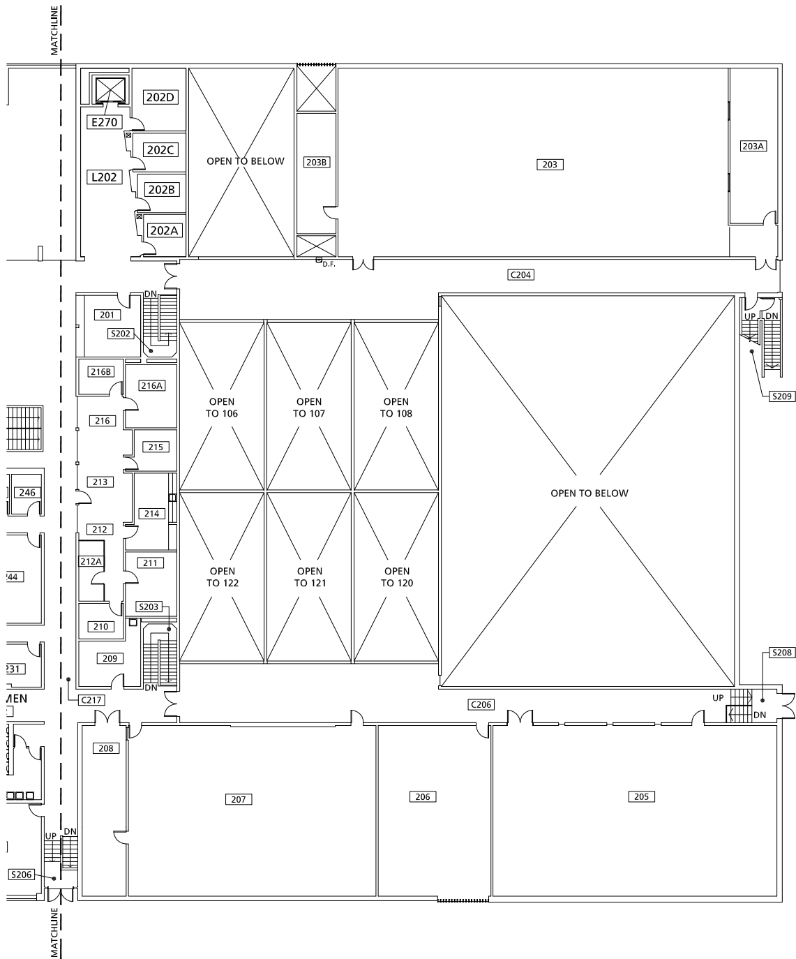
SECOND FLOOR PLAN (EAST)
