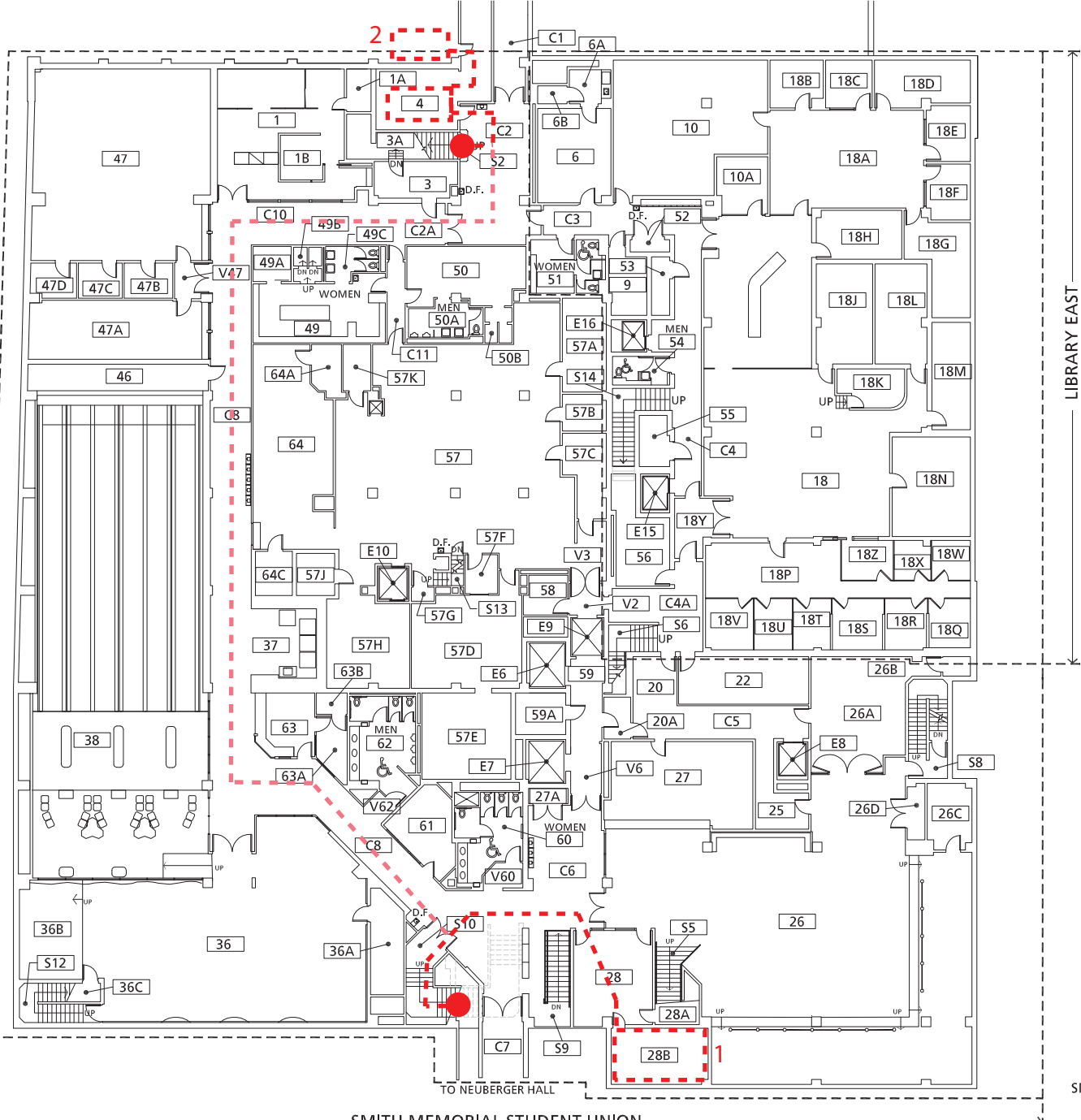
BASEMENT FLOOR PLAN (SMSU)
