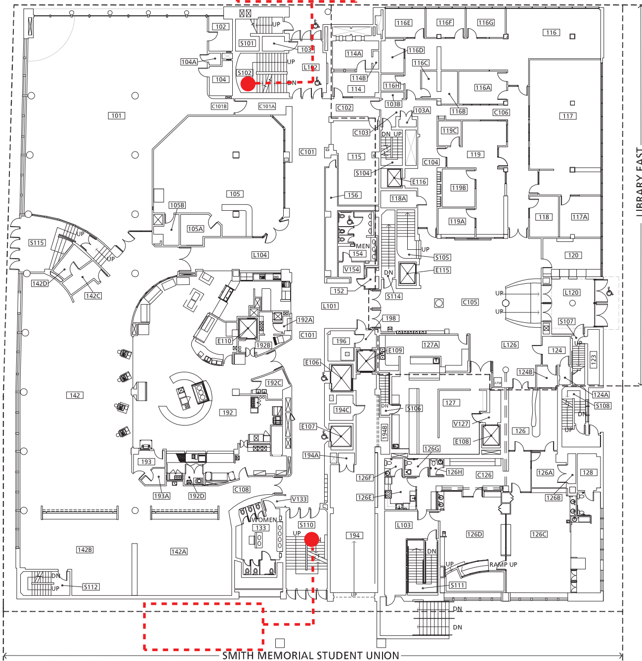
FIRST FLOOR PLAN (SMSU)
