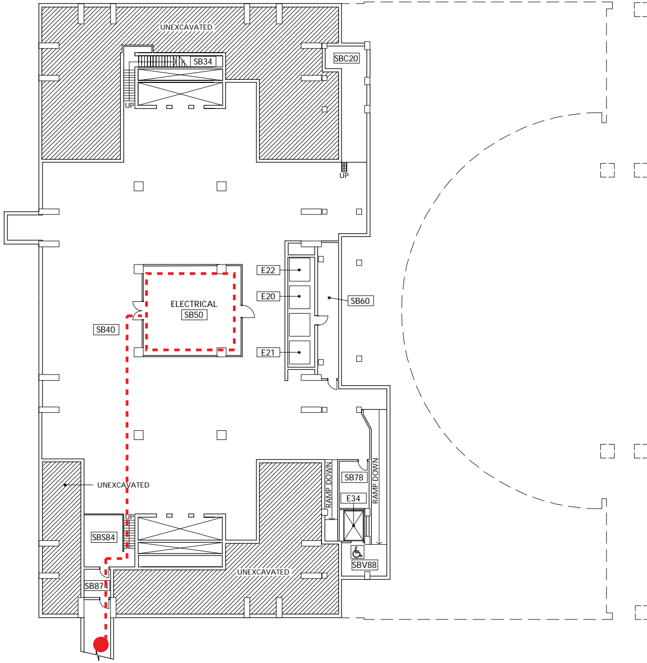
SUB-BASEMENT FLOOR PLAN
